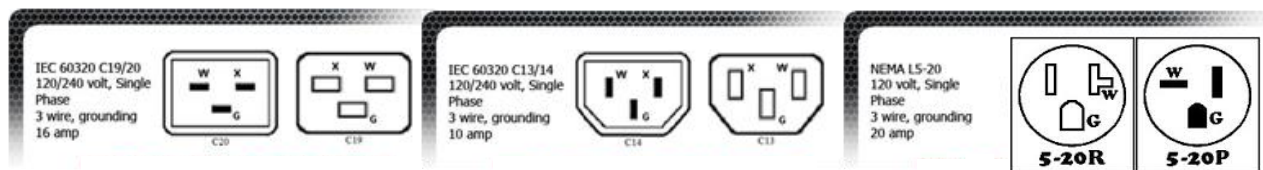
(Figure 13) – Standard Power Cable Connectors
