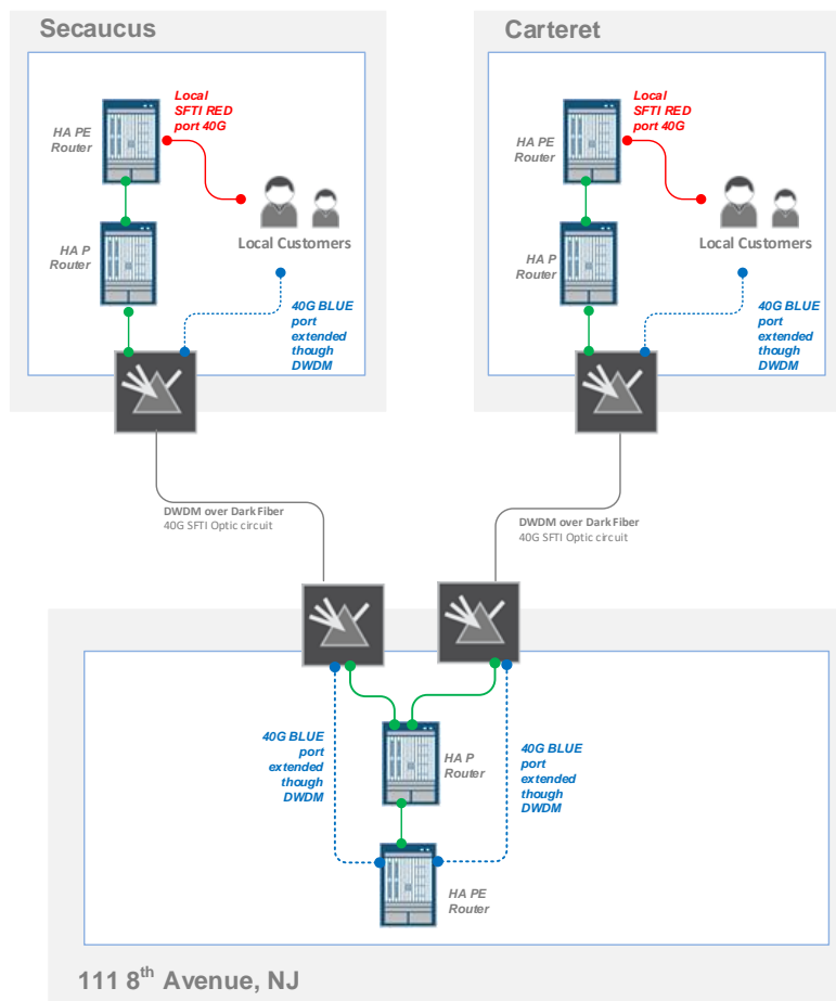
Figure 8 – 40G Bundle
